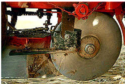
No-till double disk opener on RJ planter
